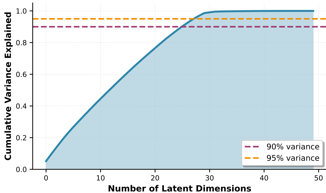
Cumulative Variance Explained
